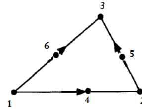
Fig. 1 Triangular element with linear edge and quadratic nodal element.
